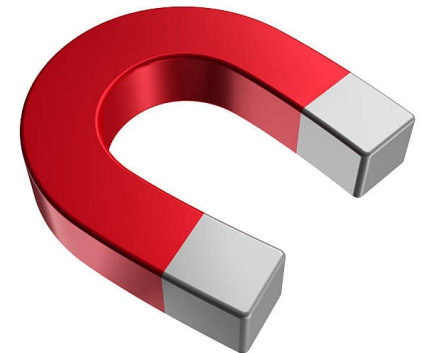
horseshoe magnet
