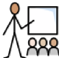
class
