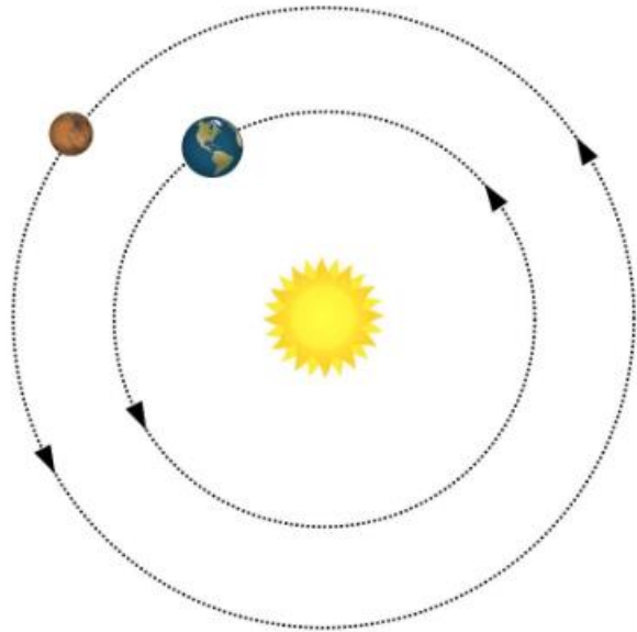
Heliocentric
