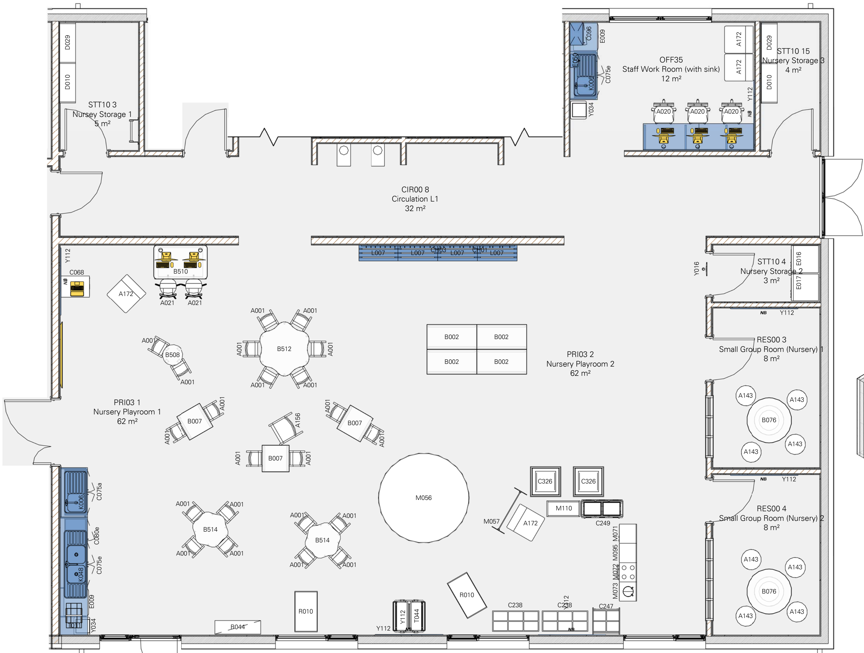
PRI03 1 - Nursery 1 : 50
