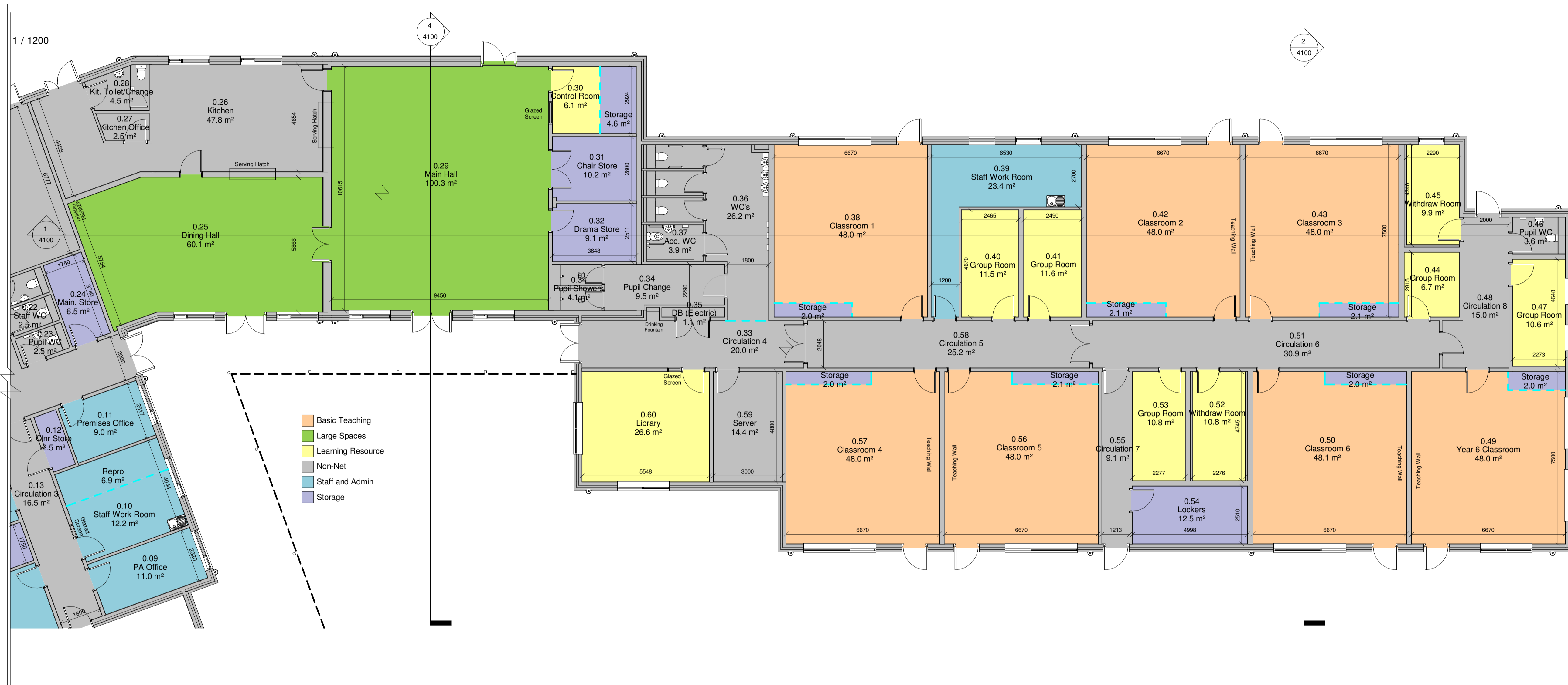
1 00(Ground) - Teaching Sheet 2 of 2 1:100
