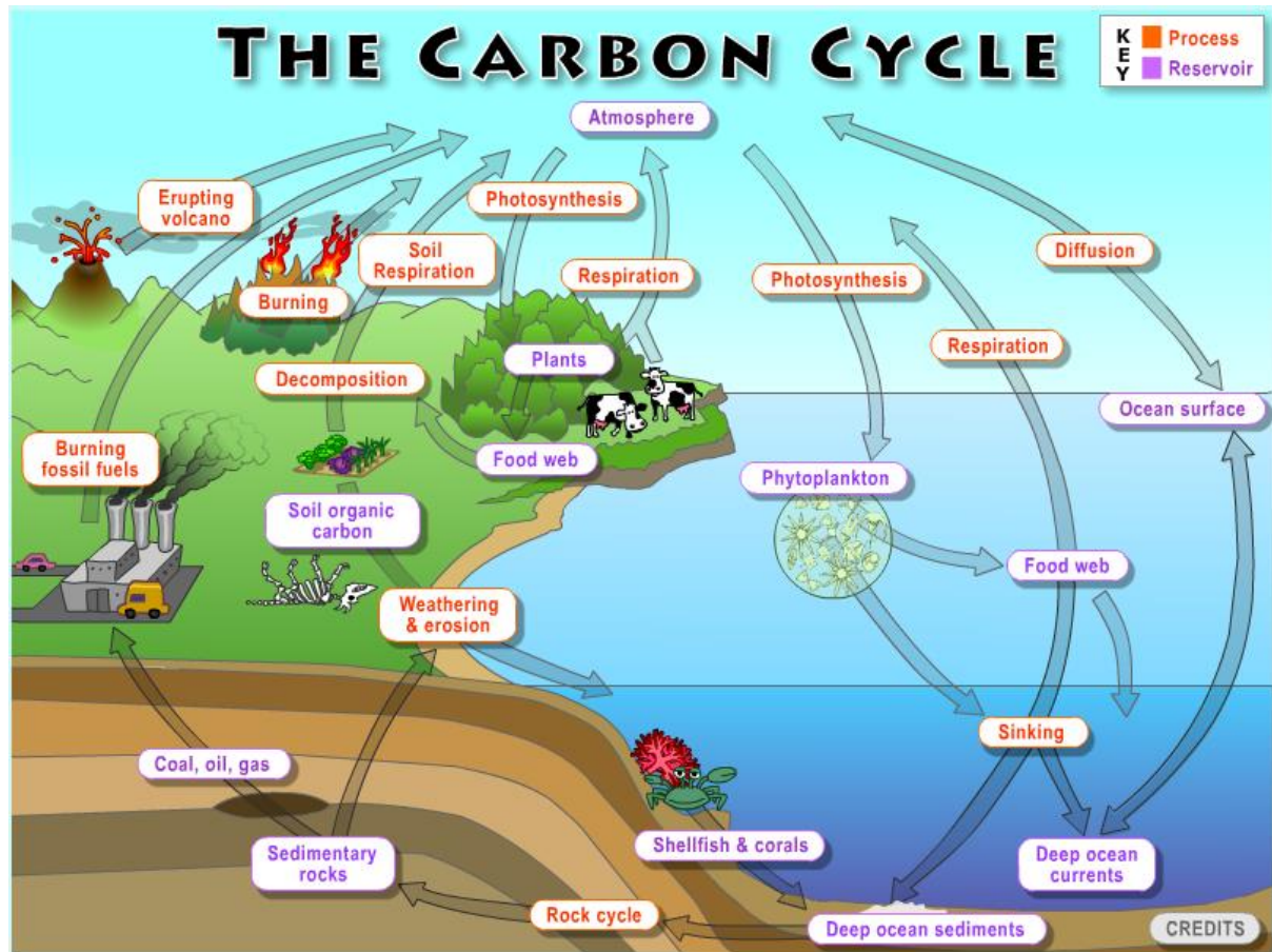
Figure 4: Some key processes which drive the flux of carbon between the main stores © Candace Dunlap. Source: http://serc.carleton.edu/eslabs/carbon/index.html
