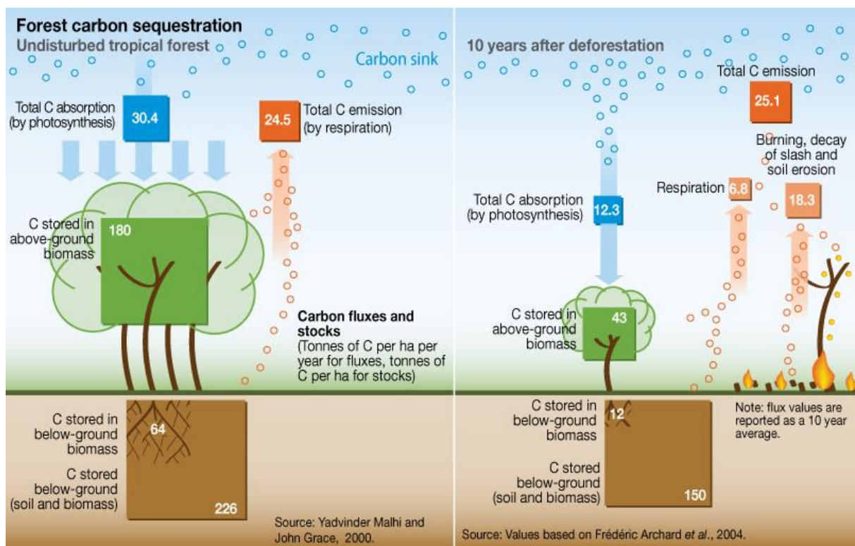
Figure 5: Changes in carbon cycling between Tropical Forest and areas of deforestation Units are tonnes of carbon per hectare per year for fluxes and tonnes of carbon per hectare for stores. Original diagram by Riccardo Pravettoni, UNEP/GRID-Arendal: http://www.grida.no/graphicslib/detail/forest-carbon-sequestration_06bd
