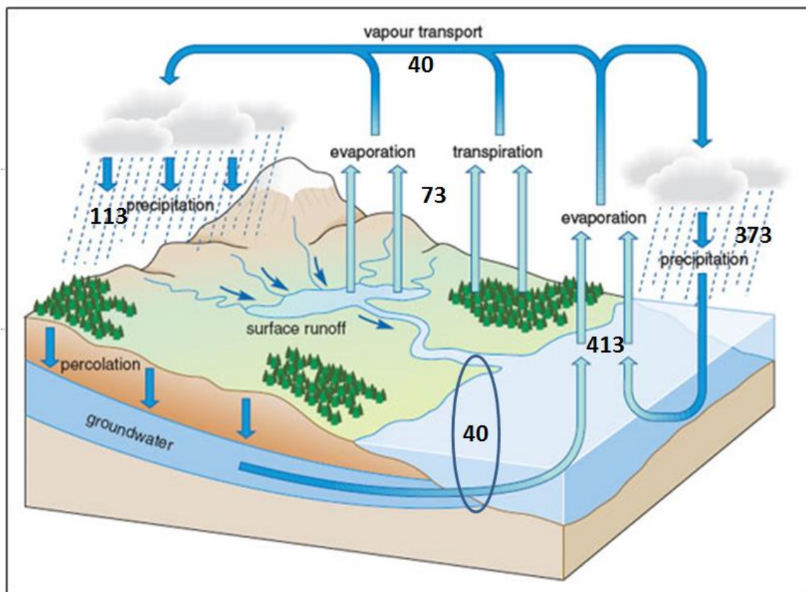
Figure 2: The global water cycle. Fluxes of moisture indicated in units of 10^3 \text{ km}^3 \text{ yr}^{-1} Original Figure © Open University Modified with data from Trenberth et al. 2007.
