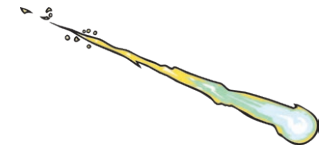
comet
