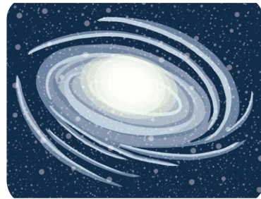
galaxy
