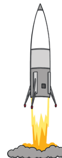
rocket
