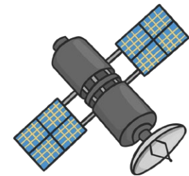
satellite
