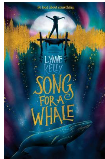
SOUND
