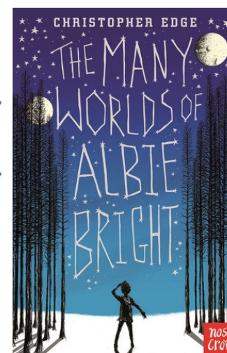
PHYSICS
