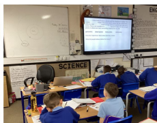
The heliocentric model
