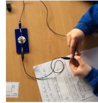
Making predictions
