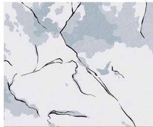
sedimentary
