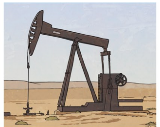
chemical fossils
