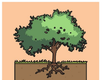
topsoil
