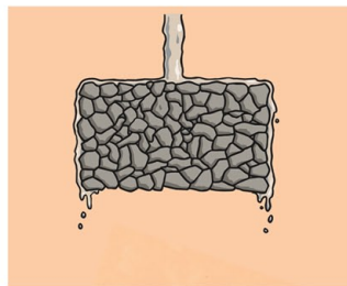
impermeable
