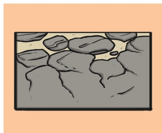
base rock
