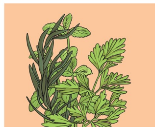
organic matter
