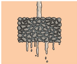
permeable
