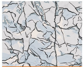
metamorphic
