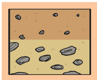
subsoil
